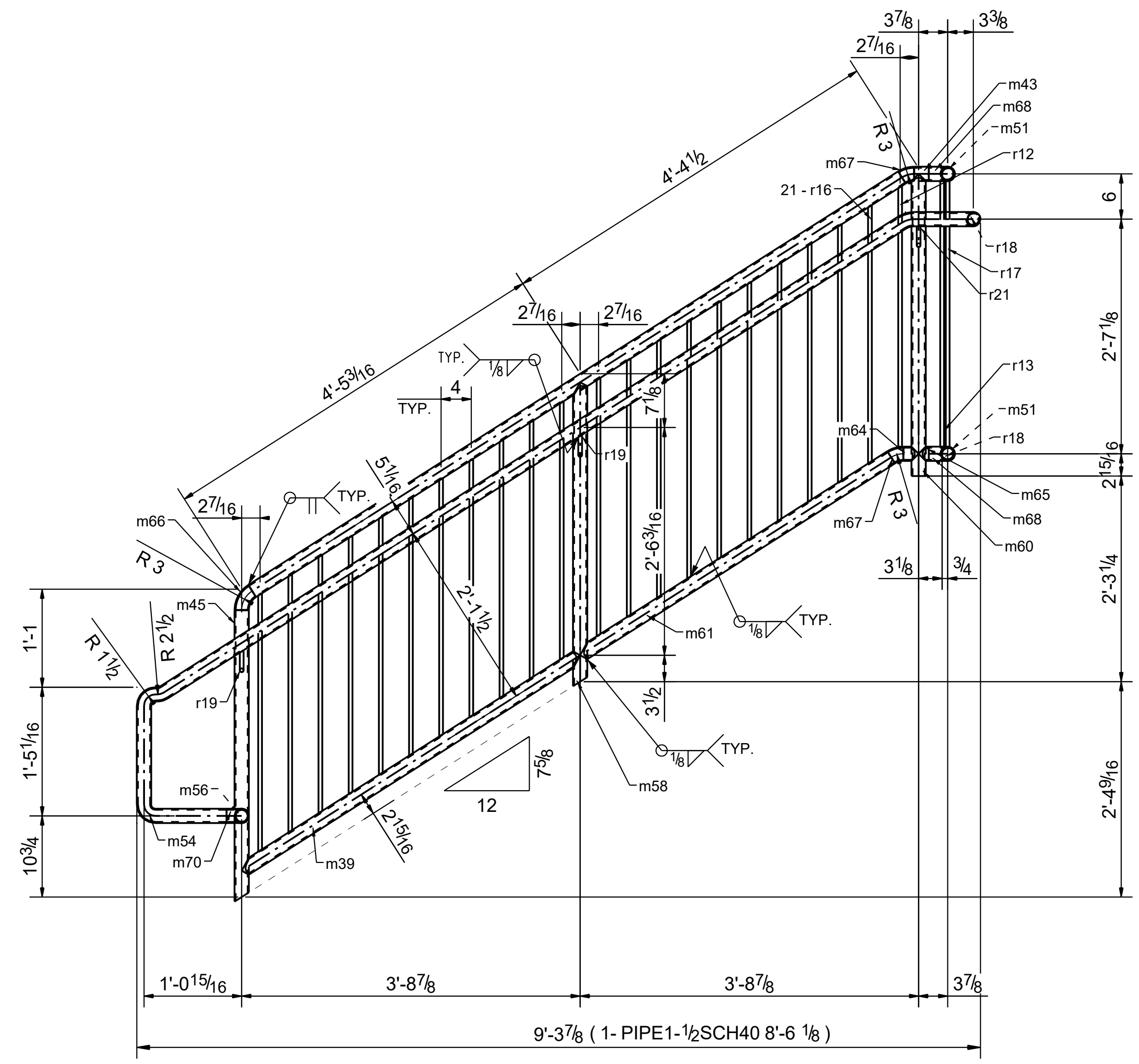
ONE - GUARDRAIL - 111GR1
