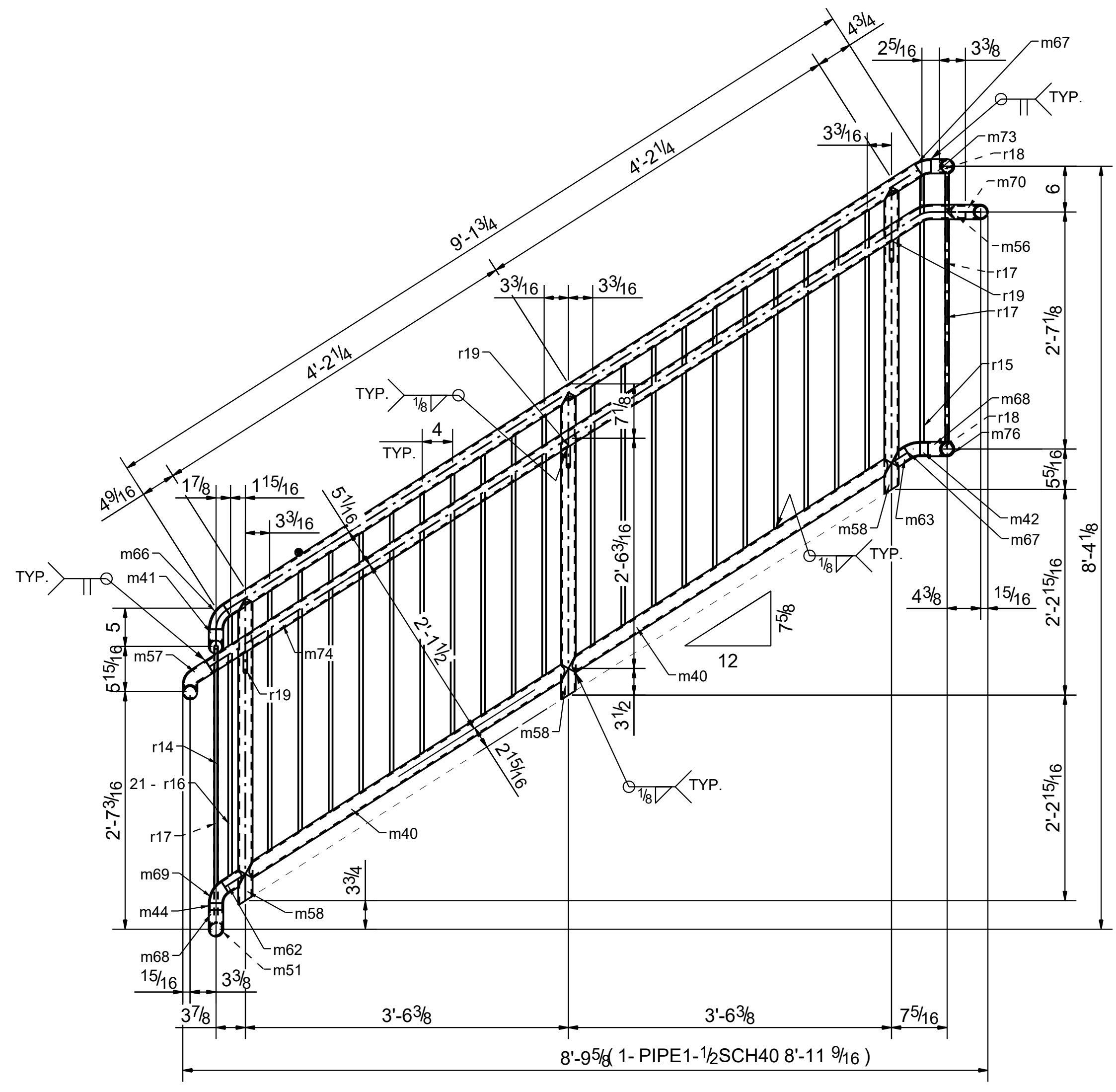
ONE - GUARDRAIL - 112GR1
