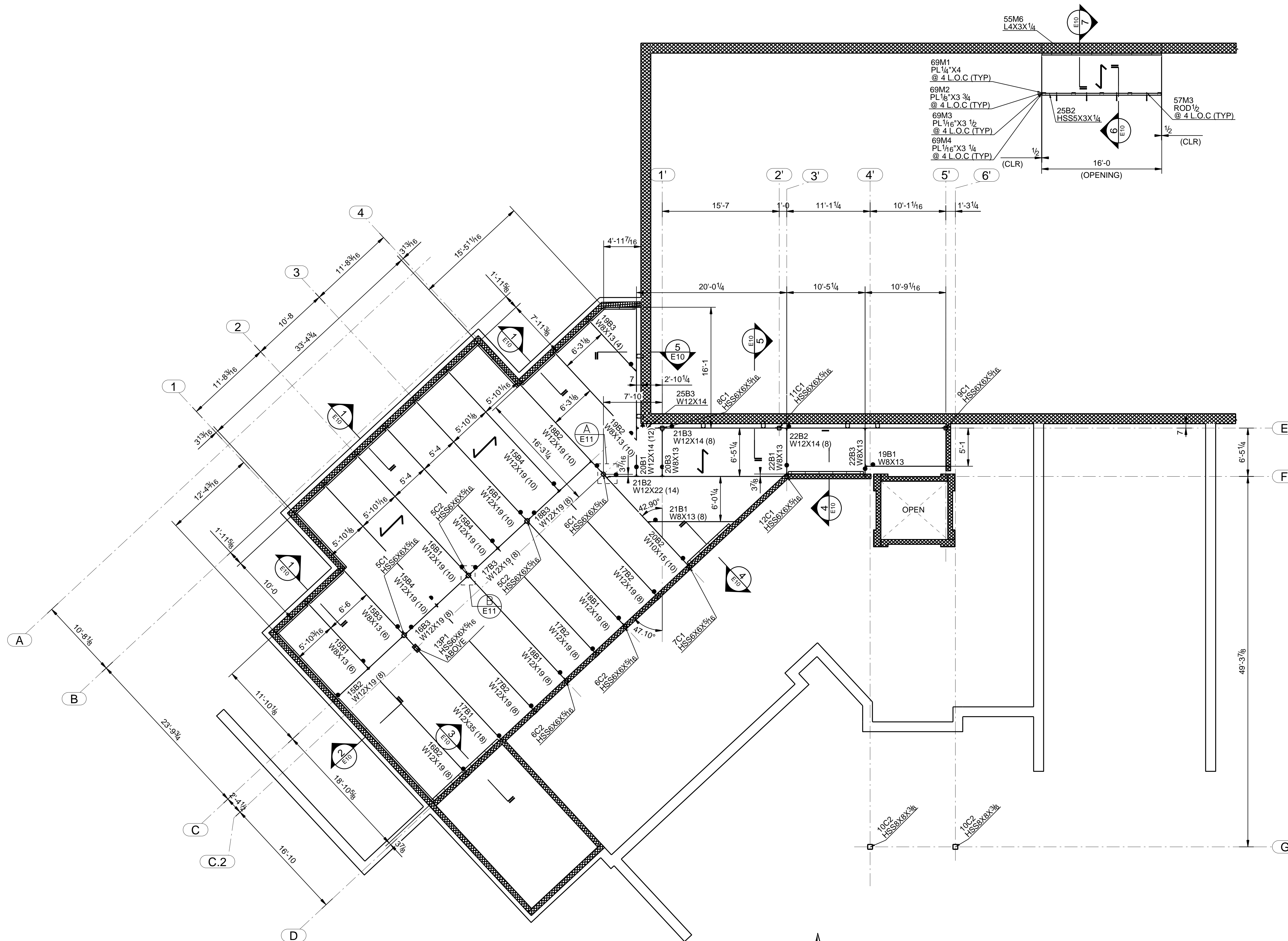
FIRST FLOOR PLAN (T.O.S EL+ 937'-3 1/2 (U.N.O))
